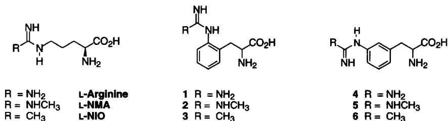
Figure 1. L-Arginine and Arginine Based NOS Inhibitors
