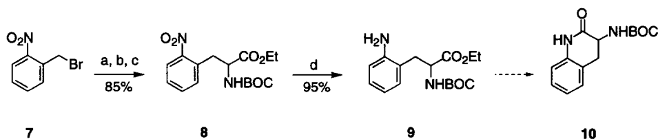
Scheme I a
