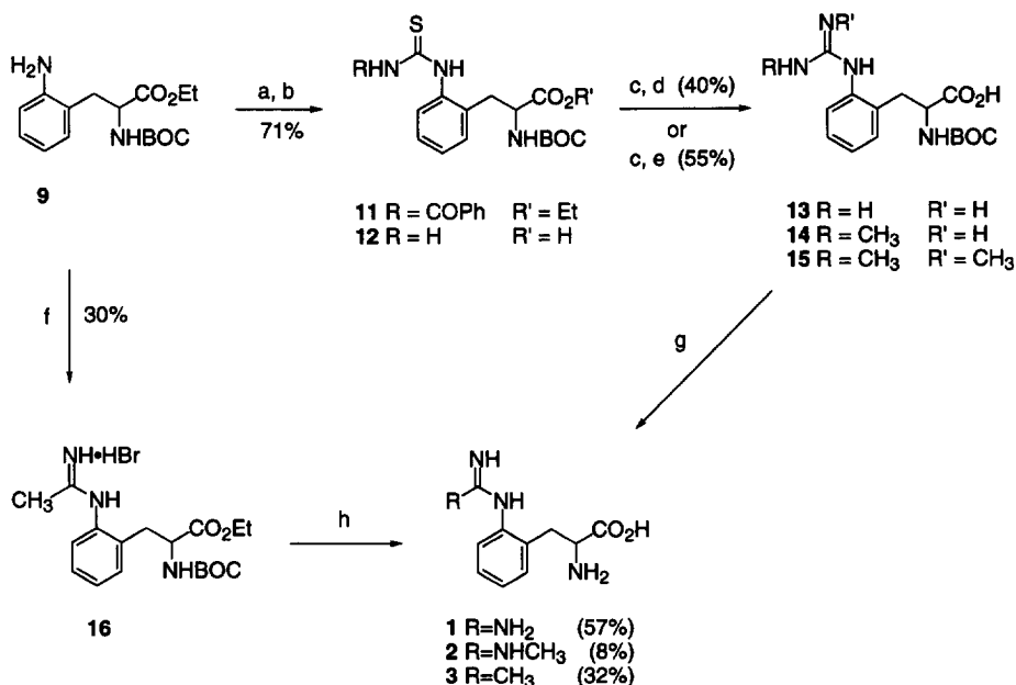
Scheme II a
