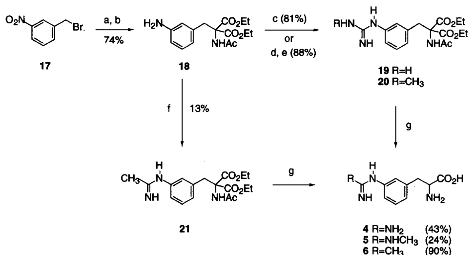
Scheme III a
